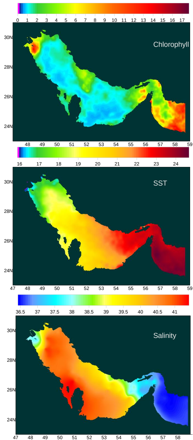
Fig. 22. Spatial distribution of the satellite derived chlorophyll (top, \mu\text{g/l} ), sea surface temperature (middle, ^{\circ}\text{C} ) and CTD in-situ salinity (bottom, psu) during February, 2006 in RSA.
