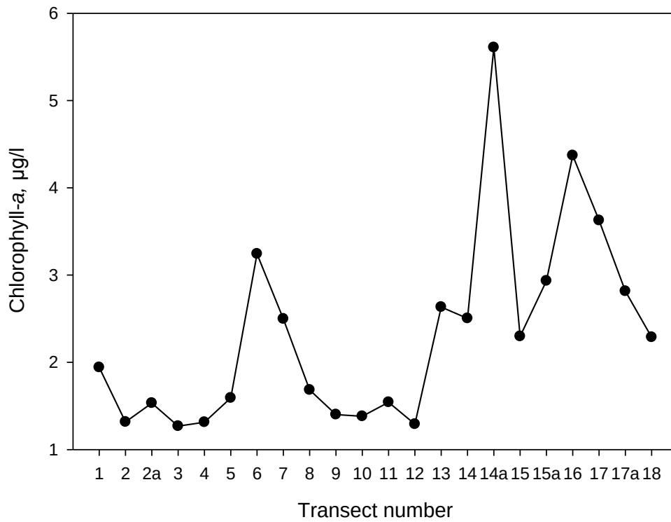
Fig. 10. Average water column concentration of chlorophyll- a (µg/l) for the different sampled transects in the RSA during Winter 2006 (transects 1-14 – Inner RSA, transect 14a – Strait of Hormuz, and transects 15-18 – Sea of Oman). Chlorophyll- a concentrations were averaged for all sampled depths per station and all sampled stations per transect.
